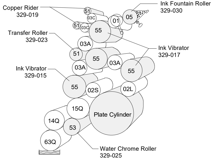
View from Operator Side with Quad Flow Dampening System
