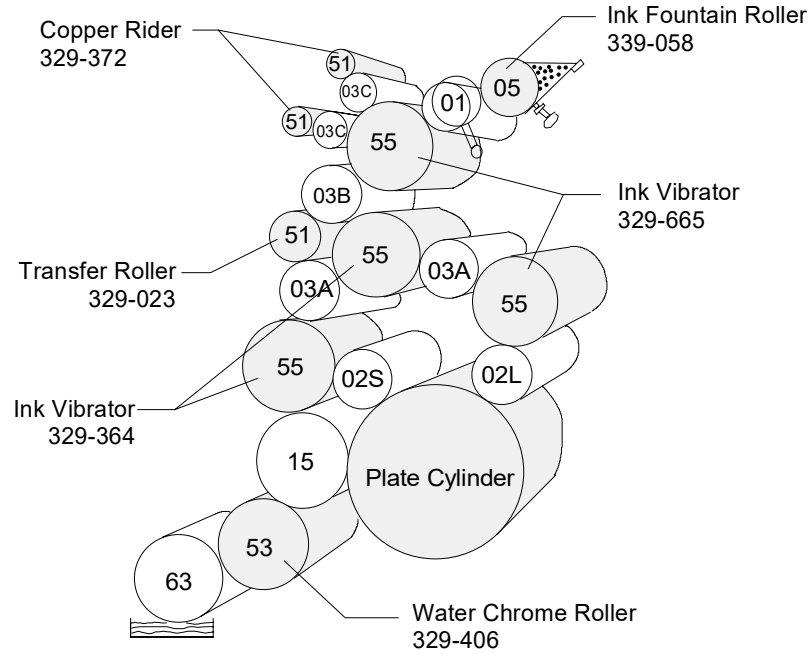
View from Operator Side (W.S.) With Tri Flow Dampening System
