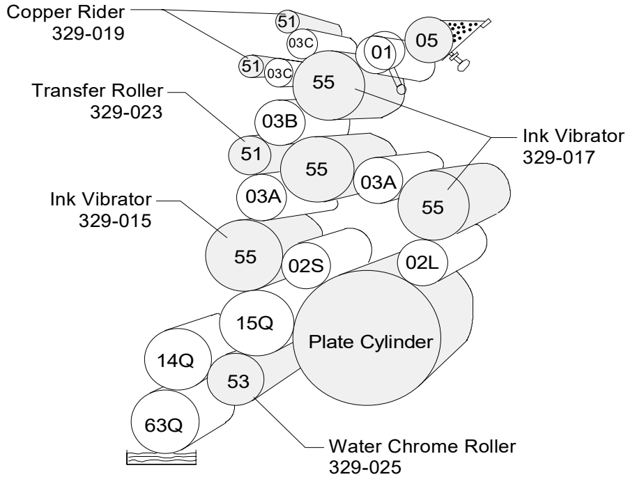
View from Operator Side With Quad Flow Dampening
