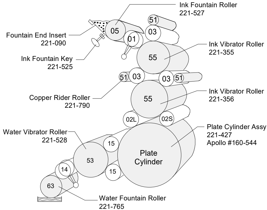
As Viewed From Operator Side (W.S.)
